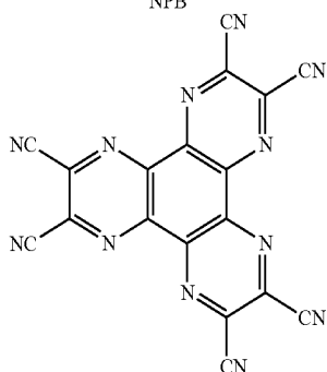
HAT—CN 6
